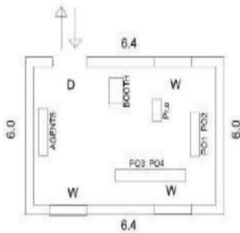
CAD View
